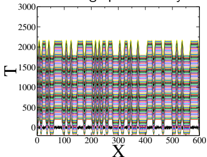
Disordered state
