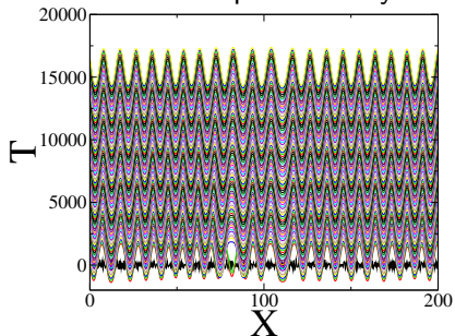
Ordered state
