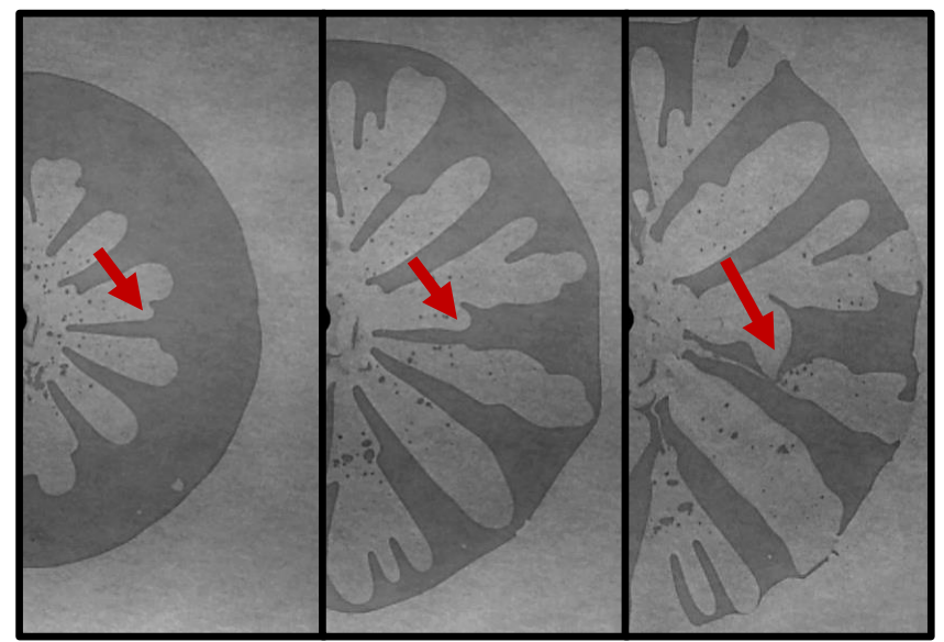
Viscous fingering
