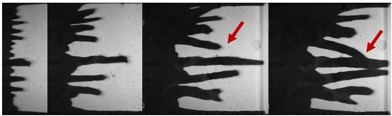
Fracture dissolution
