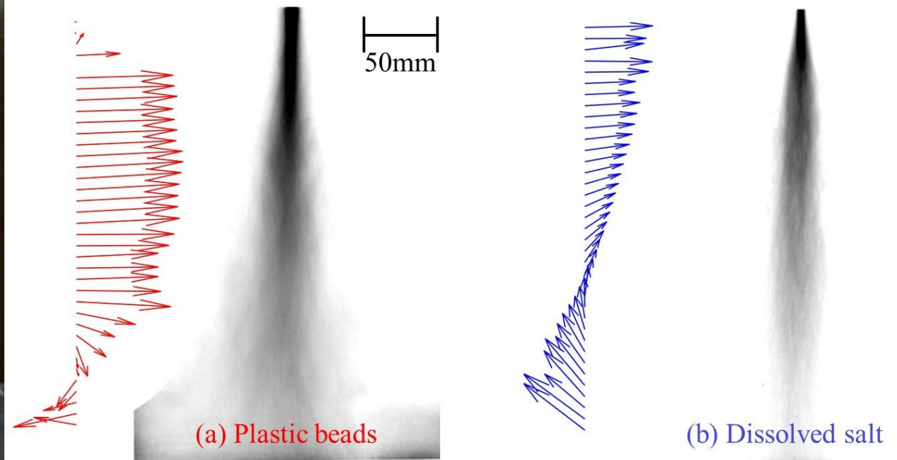
Figure 2 Average plume shape and entrainment velocity
