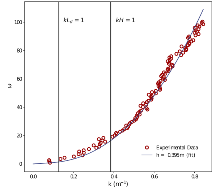
Relation dispersion according to hydro-elastic theory
